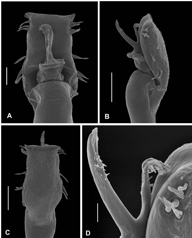
Figure 7.— Discocyrtus flavigranulatus B. Soares, 1944, male from Poços de Caldas (MNRJ 9279), penis, distal part: A. Dorsal view; B. Lateral view; C. Ventral view; D. Detail of stylus and ventral process, lateral view. Scale bars = 50 \mu\text{m} (A); 100 \mu\text{m} (B, C); 20 \mu\text{m} (D).
