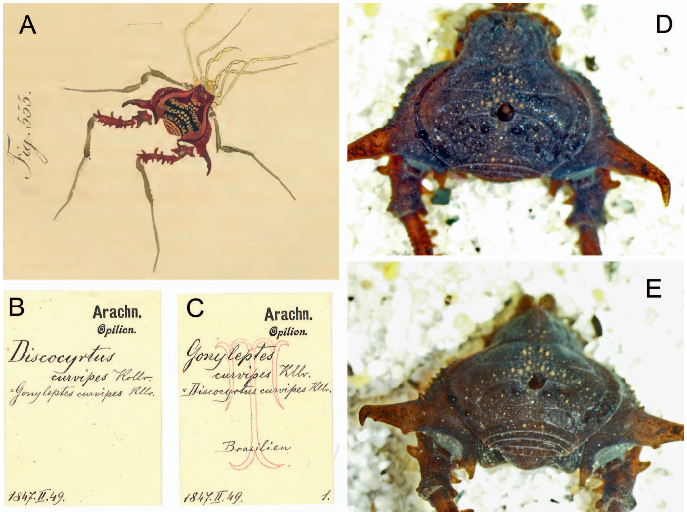
Figure 1.— Discocyrtus flavigranulatus B. Soares, 1944, male holotype of synonym Discocyrtus curvipes (Kollar in C.L. Koch, 1839), from “Brazil” (NHMW 1847.II.49, currently NHMW 3127): A. Original illustration by C.L. Koch; B. Old catalogue index card after Sørensen with the transfer from Gonyleptes to Discocyrtus ; C. Cross-reference old catalogue index card after Sørensen; D. Specimen, dorsal scutum, dorsal view; E. Same, dorso-posterior view.
