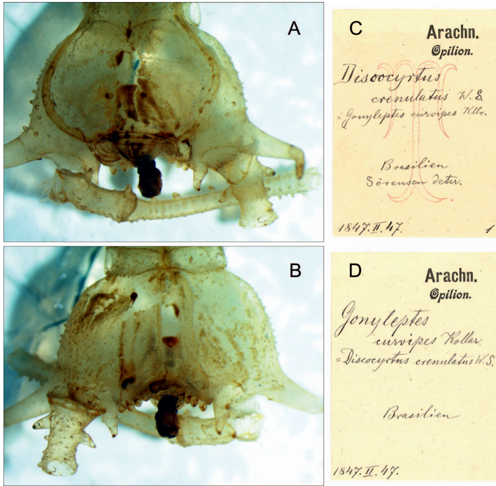
Figure 3.— Discocyrtus crenulatus Roewer, 1913, male, second specimen of Gonyleptes curvipes of Koch from “Brazil” (NHMW 1847.II.47, currently NHMW 3126), not used in the description, but regarded as a syntype of D. crenulatus by Roewer: A. Dorsal scutum, partial, and basal legs, dorsal view; B. Coxa IV, stigmatic area and basal leg IV, ventral view; C. Old catalogue index card after Sørensen with the indication of the new species in Discocyrtus crenulatus ; D. Cross-reference old catalogue index card after Sørensen.
