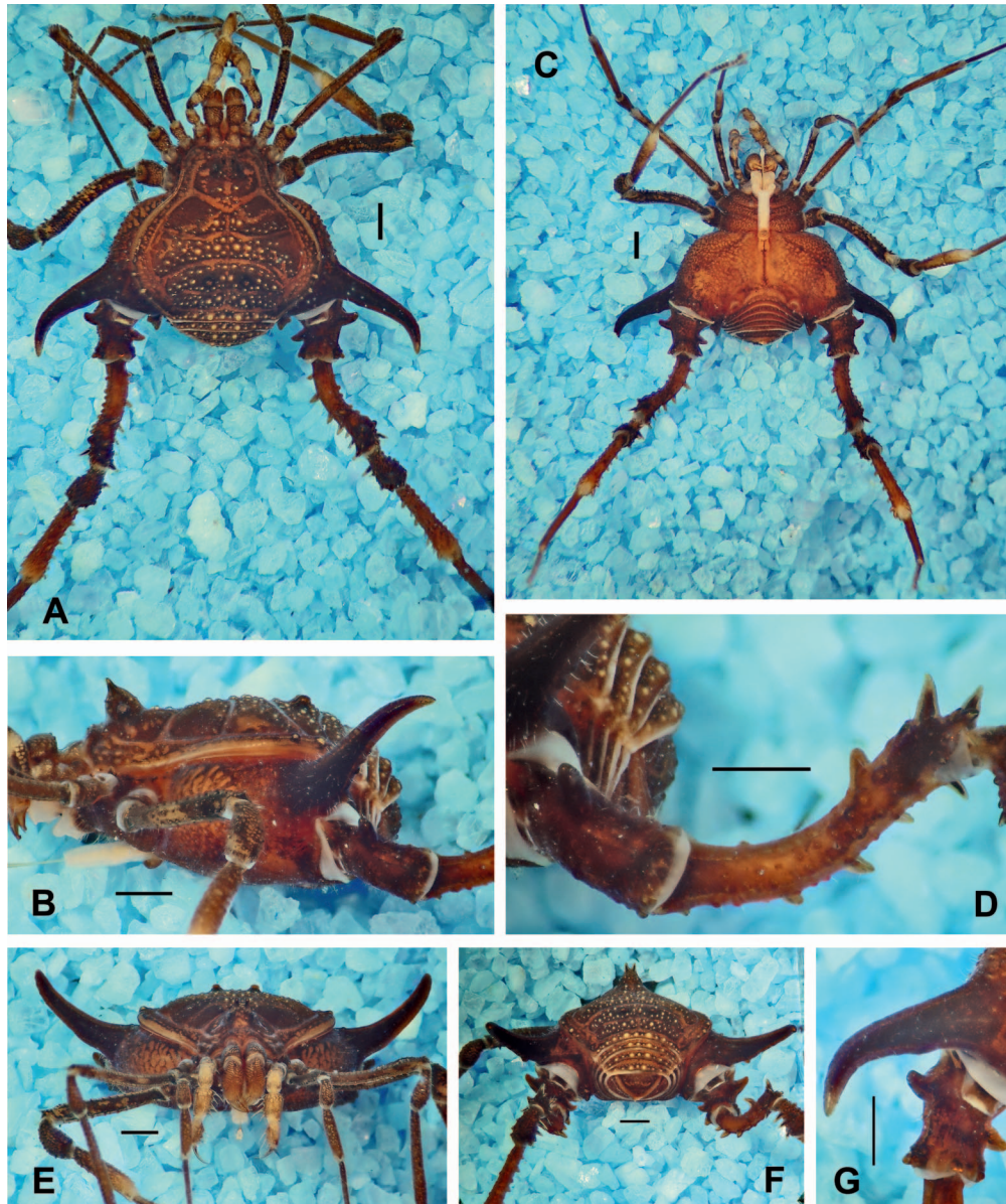
Figure 6.— Discocyrtus flavigranulatus B. Soares, 1944, male from Poços de Caldas (MNRJ 4503): A. Habitus, dorsal view; B. Same, lateral view; C. Same, ventral view; D. Tr and Fe IV, prolateral view; E. Habitus, anterior view; F. Same, posterior view; G. Cx IV, prodorsal distal apophysis. Scale bars = 1 mm.
