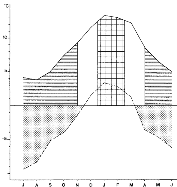
Fig. 2: Climatic diagram for the locality of El Cónдор, Pampa de Achala (1973–1978). Squared area=intermediate season without frosts, white area=intermediate season with frosts, hatched area=thermic winter, dotted area=frost period. Solid curve=mean temperatures, dashed curve=absolute minimum temperatures.
